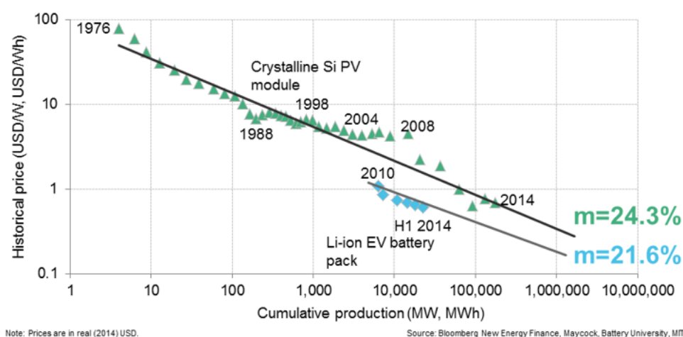
Figure 7: Solar PV and Lithium Ion experience curve comparison 25
