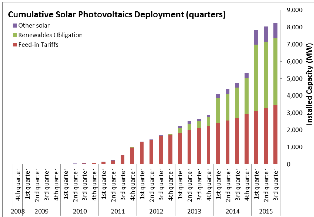
Figure 3: Solar PV cumulative capacity in UK, 2008 to Q3 2015
